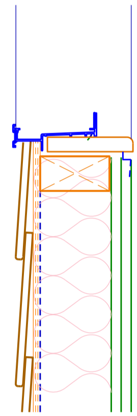
TYPE 06 Weatherboard two layers of 13mm plasterboard internally
