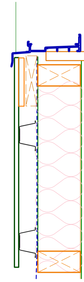
TYPE 12 Cemintel Barestone - 35mm furring channels, two layers of 13mm plasterboard internally
