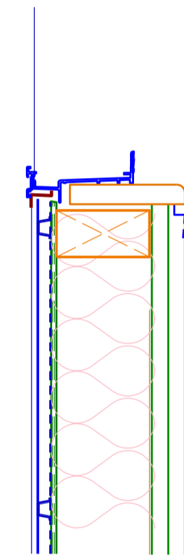
TYPE 08 Mini-Orb - 12mm furring channels, 1 layer 6mm fibre cement externally two layers layer of 16mm plasterboard internally
