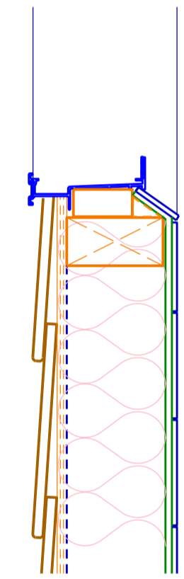
TYPE 07 Weatherboard one layer of 6mm Fibre cement and tiles internally one layer of 13mm plasterboard internally
