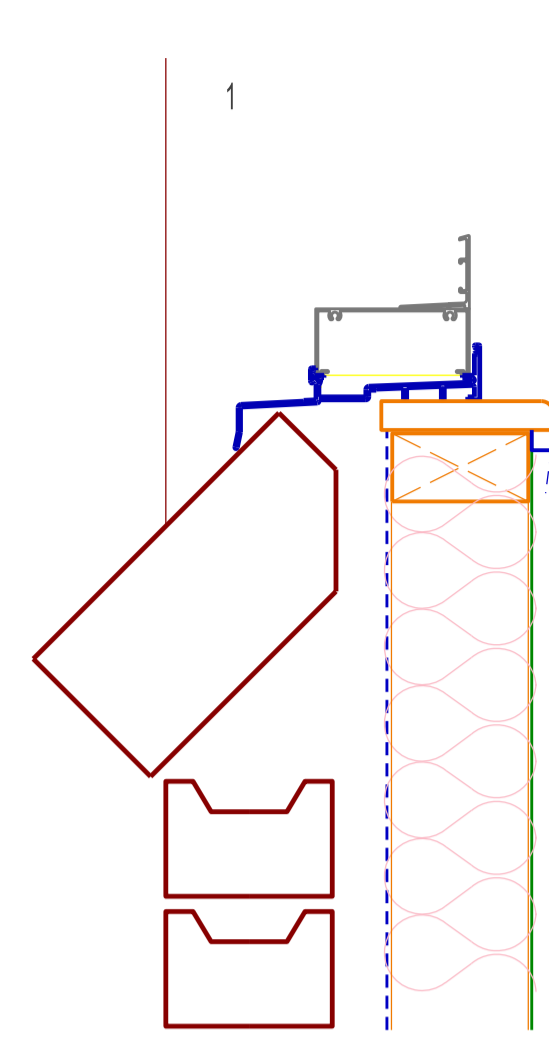
TYPE 03 Brick Veneer - Brick on edge sill one layer of 13mm plasterboard internally
