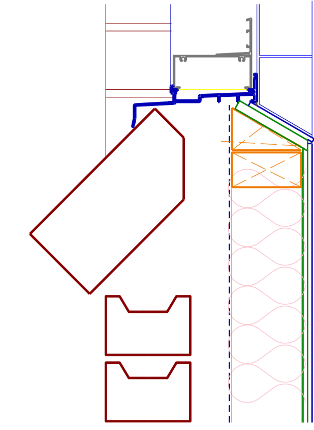
TYPE 15 Brick Veneer - Brick on edge sill one layer of 6mm fibre cement and tiles internally
