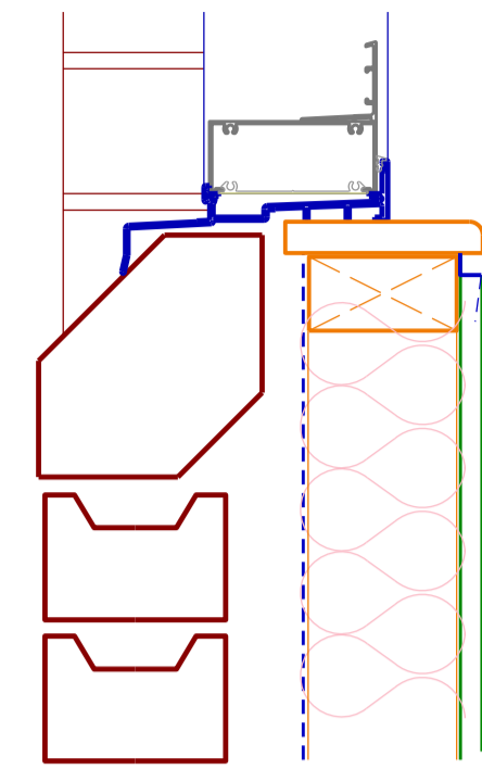
TYPE 02 Brick Veneer - Cant sill one layer of 13mm plasterboard internally
