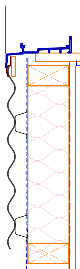
TYPE 10 Custom Orb - 25mm furring channels, two layers layer of 13mm plasterboard internally
