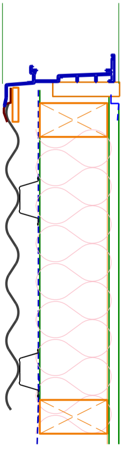
TYPE 11 Custom Orb - 25mm furring channels, one layer of 13mm plasterboard internally
