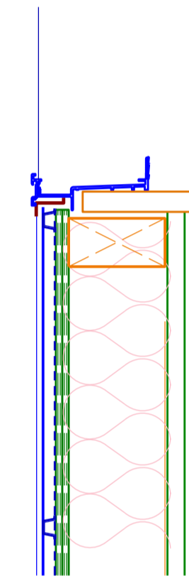
TYPE 09 Mini-Orb - 12mm furring channels, 2 layers 6mm fibre cement externally two layers layer of 16mm plasterboard internally
