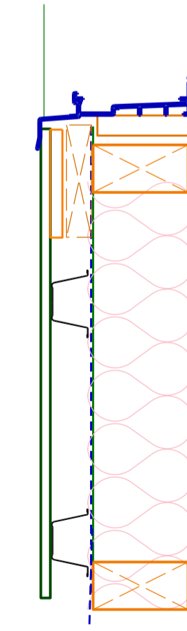
TYPE 14 Cemintel Barestone - 35mm furring channels, one layer of 6mm fibre cement internally
