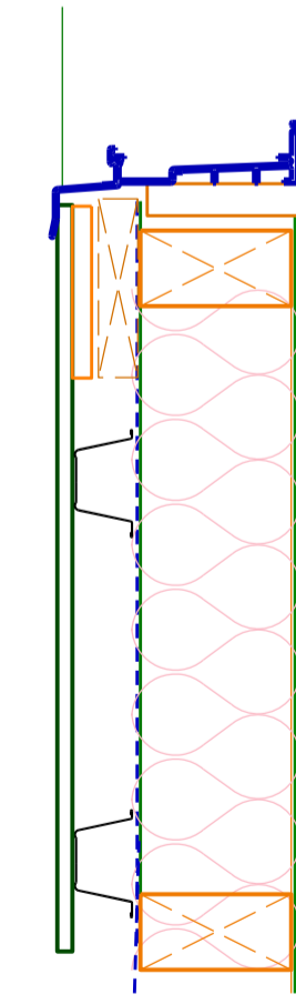
TYPE 13 Cemintel Barestone - 35mm furring channels, one layer of 13mm plasterboard internally
