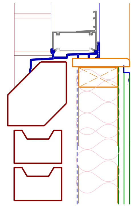
TYPE 01 Brick Veneer - Cant sill two layers of 13mm plasterboard internally
