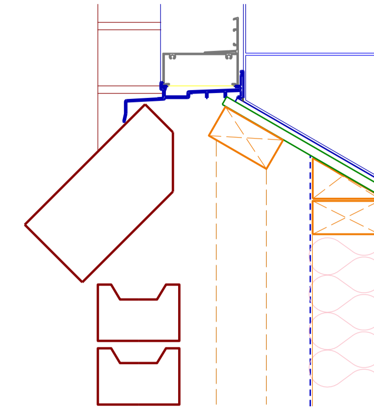
TYPE 05 KITCHEN WINDOW - cavity width varies Brick Veneer - Brick on edge sill one layer of 6mm fibre cement and tiles internally
