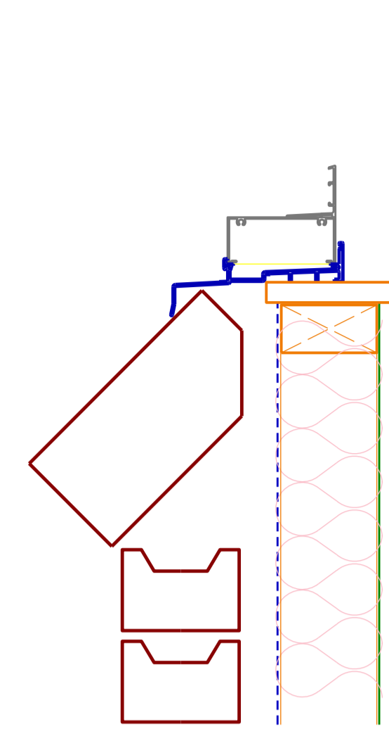
TYPE 04 Brick Veneer - Brick on edge sill two layers of 13mm plasterboard internally
